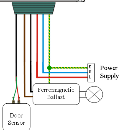
Connection Diagram
